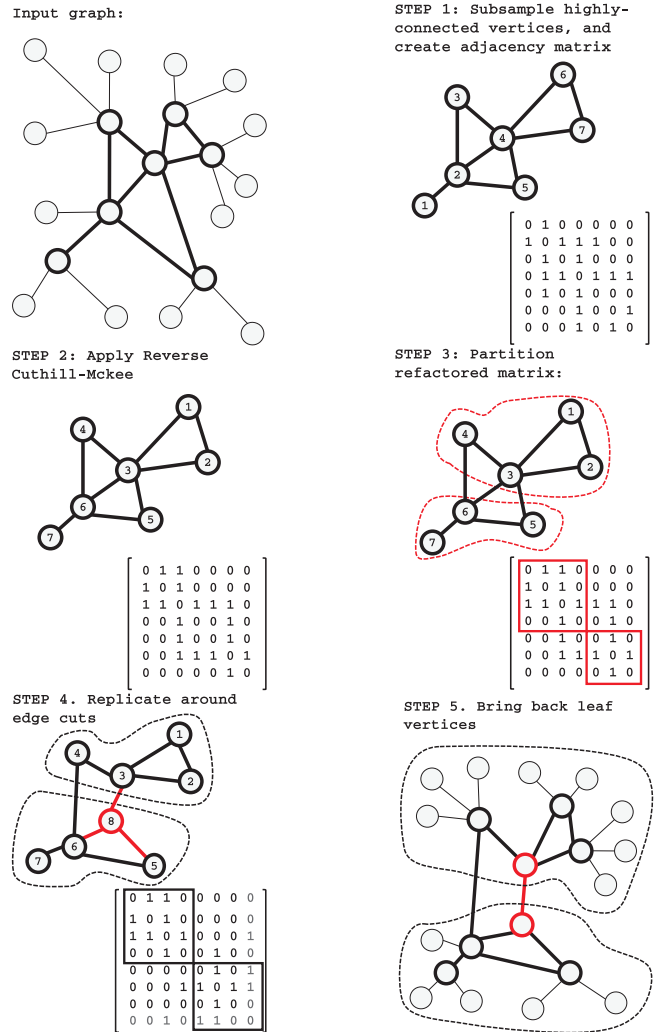
Figure 3: Example algorithm
