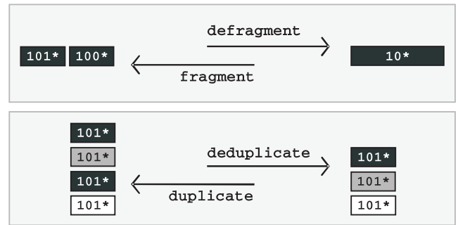
Figure 6: Reduce transformations
